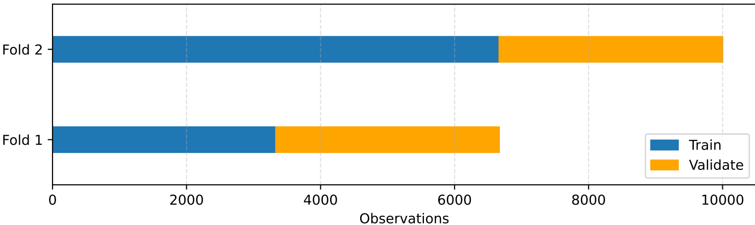
Expanding Time Series Cross-Validation (TSCV)
